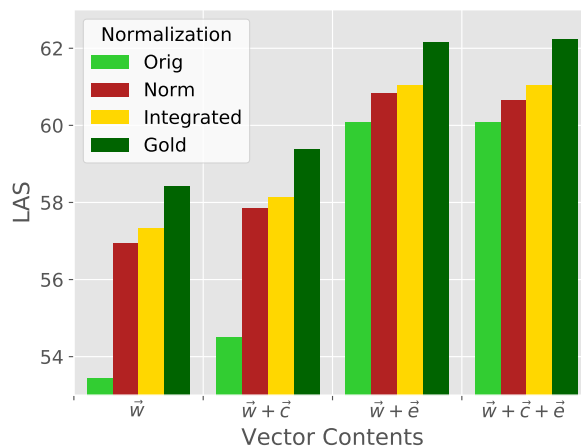
Figure 2: The effect of normalization on LAS for the different parsing models on the development data.
