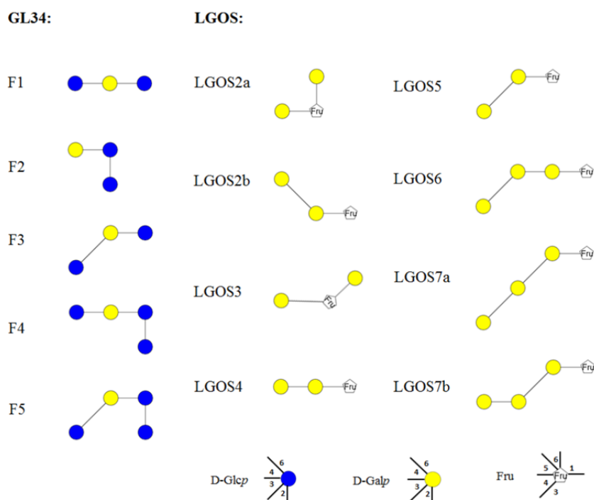
Scheme 1: Schematic presentation of all structures in the GL34 glucosylated-lactose (lactose = galactosyl-glucose) and LGOS galactosylated-lactulose (lactulose = galactosyl-fructose) mixtures used. 20,21
