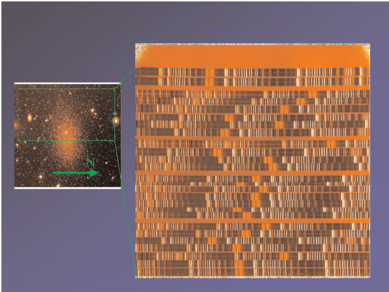
Figure 2: A FORS1 R-band image of Tucana taken in August 1999. The green outline shows the region covered by the MXU slit mask, and thus the region where spectra were obtained. The CCD image on the right is the raw spectra on one of the two FORS2 CCDs (the “master” CCD) for our spectra of stars in Tucana.
