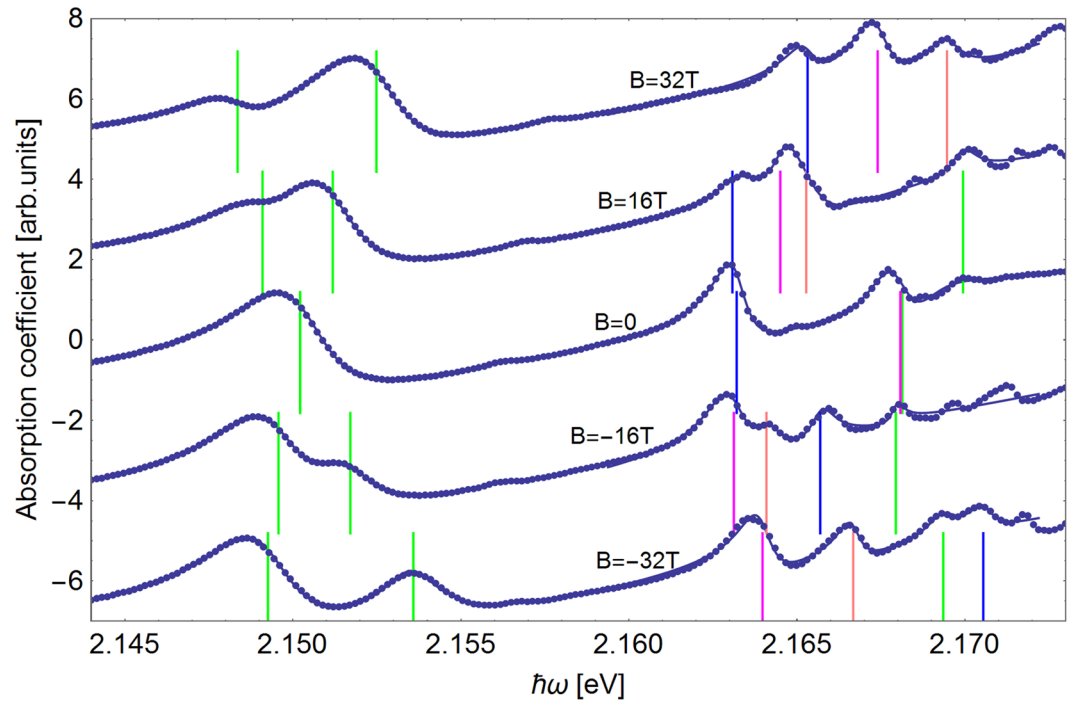
Figure 4. The absorption spectrum for the n=2, 3 exciton (dots) at various values of magnetic field fitted with the sum of asymmetric Lorenzian peaks (solid line). The 'bare' exciton energies (see text) are indicated by vertical lines. The fit quality parameter is R^2 > 0.999997 for the n=2 levels and R^2 > 0.9996 for n=3 levels.
