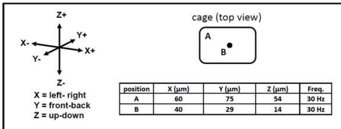
Figure 1: Peak to peak displacement in \mu\text{m} , measured in the corner (position A) and center (position B) of the cage (black dot in cage top view indicates the connection to the underlying oscillator).
