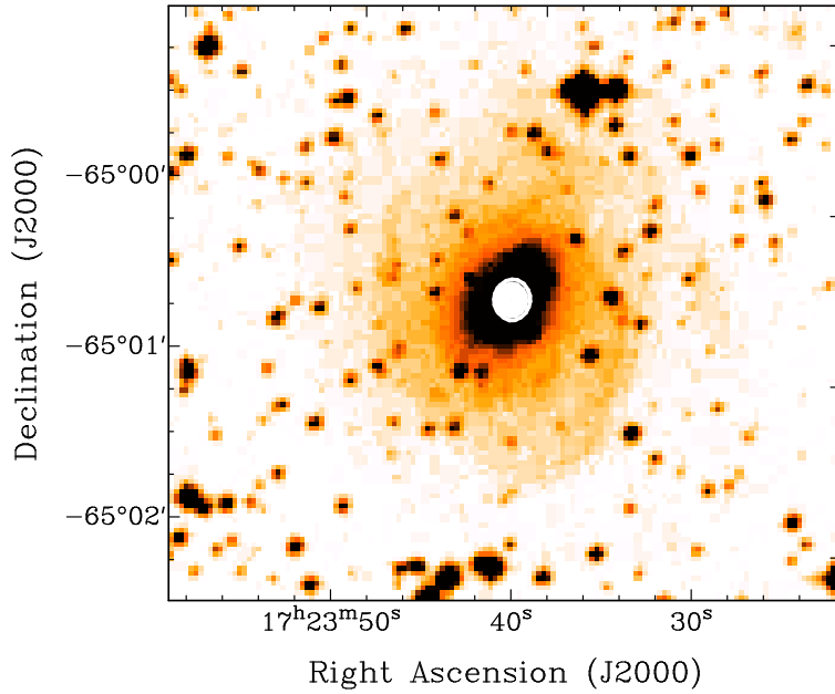
Fig. 4.2: I-band Image of PKS B1718–649: the spiral arms form an envelope around the elliptical like central part of the galaxy [UKSchmidt telescope, DSS, 1993 (NED)]. The unresolved radio source is marked in white.
