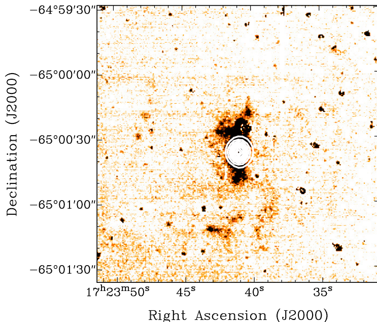
Fig. 4.3: H_{\alpha} image of PKS B1718–649 from the CTIO 1.5 m telescope. The field is 2.3' \times 2.3' with North at the top. A complex extended emission region is visible, with a strong concentration N-S from the nucleus. An extensive filamentary structure seems to follow the spiral structure seen in the I band (Keel & Windhorst, 1991). The unresolved radio source is marked in white.
