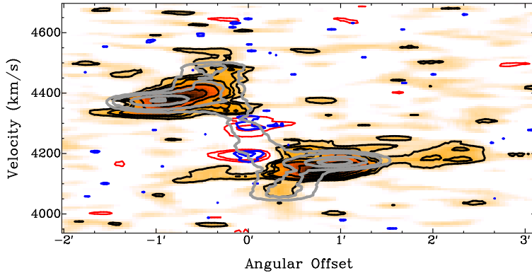
Fig. 4.9: Position-velocity plot of the H I emission disk (black) compared to the tilted ring model, smoothed at the resolution of the observations (grey contours). The contour levels range between 1.7 \text{ mJy beam}^{-1} and 7 \text{ mJy beam}^{-1} , with steps of 1.4 \text{ mJy beam}^{-1} . The model describes a regularly rotating disk, with a warp in the inner part, oriented along the N-S axis. The two absorption features are shown in blue and red, at the resolutions of 11'' and 30'' . Contour levels are -2, -8 \text{ mJy beam}^{-1} and -1.7, -3.5 \text{ mJy beam}^{-1} , respectively.
