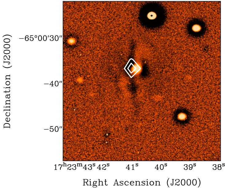
Fig. 4.4: Detail of the GUNN-I observation of PKS B1718–649. An absorbed thin disk of dust is oriented in the N-S direction. We applied unsharp masking to the image to better highlight the dust lane [Veron-Cetty et al. 1995]. The unresolved radio source is marked in white.
