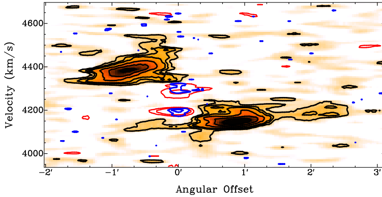
Fig. 4.6: Position-velocity plot along a slice taken at PA= 108^\circ of the H I disk. In black is shown the emission. The contour levels range between 1.7 \text{ mJy beam}^{-1} and 7 \text{ mJy beam}^{-1} , with steps of 1.4 \text{ mJy beam}^{-1} . The absorption features are circled in blue and red, at the resolutions of 11'' and 30'' . Contour levels are -2, -8 \text{ mJy beam}^{-1} and -1.7, -3.5 \text{ mJy beam}^{-1} , respectively. The blue-shifted emission shows an external ‘plume’ of the disk (in the NW of the total intensity map), at lower densities with respect to the regularly rotating ring.
