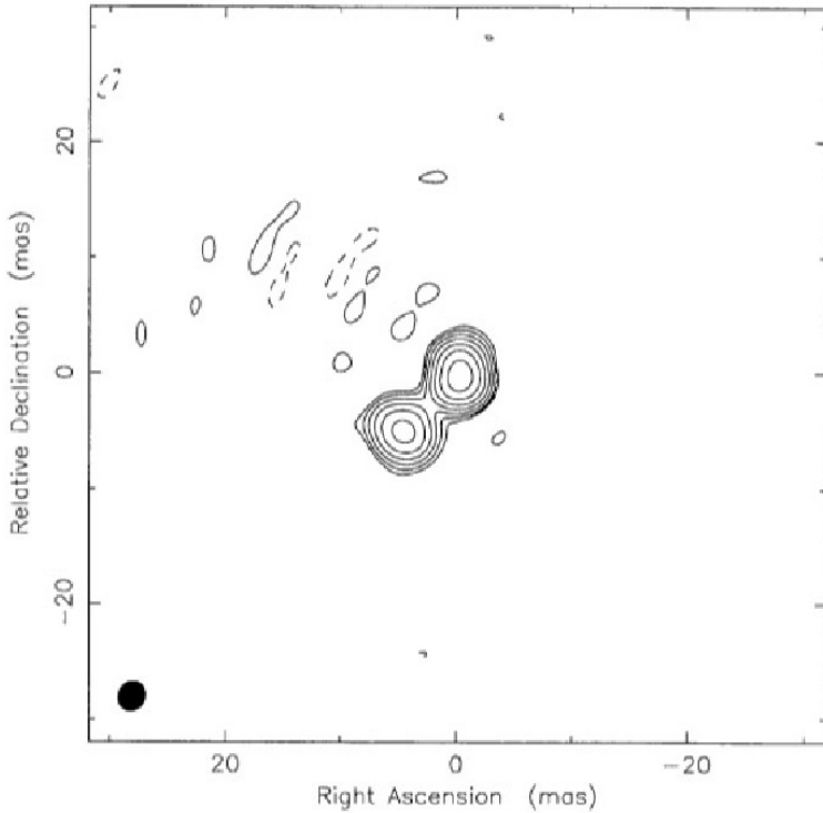
Fig. 4.1: 4.8 GHz SHEVE VLBI image of PKS B1718–649. The contour levels shown are -1,1,2,4,8,16,32 and 64% of the peak flux density of 2.0 Jy. The restoring beam FWHM dimensions are 2.6x2.3 mas, the major axis position angle is -29.5^\circ (Tingay et al., 1997).
