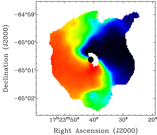
Fig. 4.7: Velocity field of the H I disk of PKS B1718–649. The position angle and inclination of the minor axis of the field varies with the radius, suggesting a warped structure of the disk in the inner regions. The color-scale ranges between 4140 \text{ km s}^{-1} and 4420 \text{ km s}^{-1} , showing the systemic velocity of the galaxy ( 4274 \text{ km s}^{-1} ) in green. The unresolved continuum radio source is marked in black.
