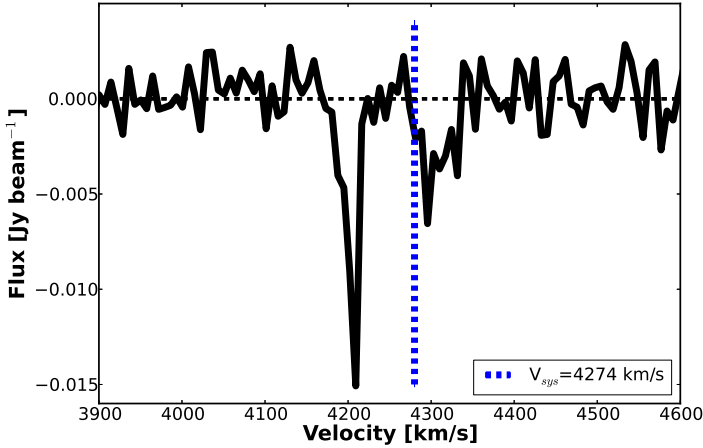
Fig. 4.8: H I profile of PKS B1718–649 obtained from the ATCA data. The two absorption systems are clearly visible. The narrow line is located at velocity 4200 \text{ km s}^{-1} , blue-shifted with respect to the systemic velocity ( 4274 \text{ km s}^{-1} , blue dashed line). The broad component is double peaked and found at velocity 4300 \text{ km s}^{-1} .
