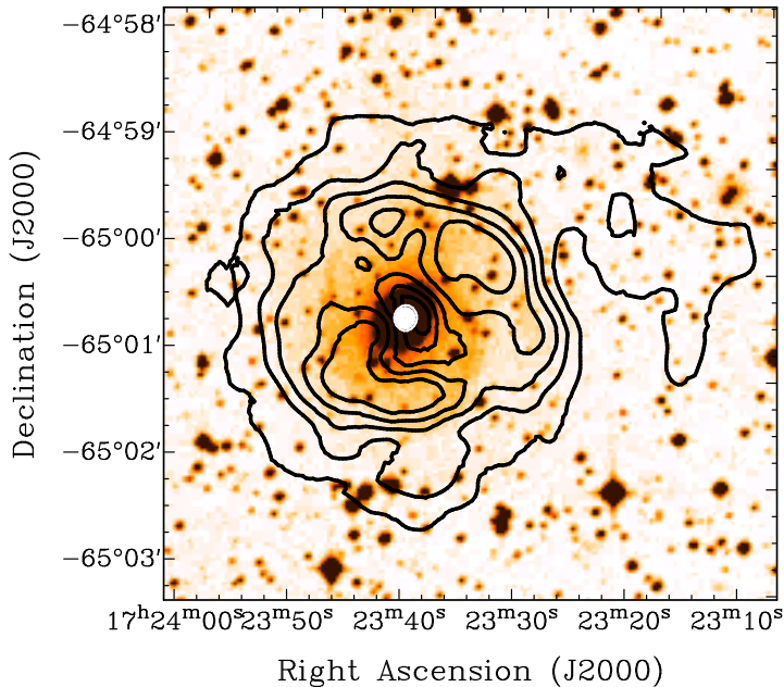
Fig. 4.5: I-band optical image of PKS B1718–649, overlaid with the column density contours (in black) of the neutral gas. The H I disk has the shape of an incomplete ring with asymmetries in the NW and in the S of the disk. The contour levels range between 7 \times 10^{19} \text{ cm}^{-2} and 8 \times 10^{20} \text{ cm}^{-2} , with steps of 1.5 \times 10^{20} \text{ cm}^{-2} . The unresolved radio source is marked in white.
