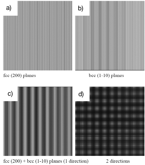
Fig. 5. Moiré fringe simulations (a) (200) planes of the fcc phase in the [001] direction, (b) (1 -1 0) planes of the bcc phase in the [001] direction, (c) overlapping in one direction with (1-10)_{bcc} // (200)_{fcc} , and (d) overlapping in two perpendicular directions.
