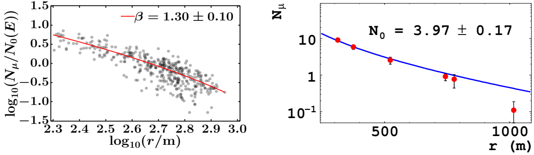
Figure 5: (Left) Muon lateral distribution for normalised data; an effective value for the slope \beta is found and can be used for individual event fits. (Right) As a preliminary result, an LDF fit fixing \beta is shown for a 10^{18.3} eV event, where only N_0 remains as a free parameter.
