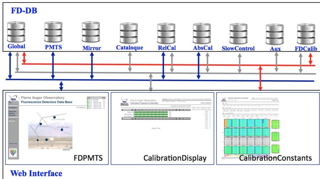
Fig. 3: The structure of the Web Graphical Interface.
