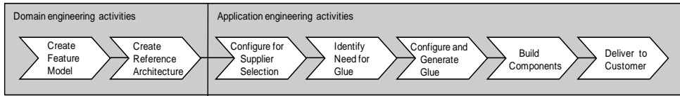
Figure 36 Process overview
