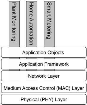
Figure 33 Layers in the ZigBee protocol with profiles
