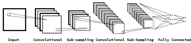
Fig. 4: The structure of a convolutional neural network. It starts with alternating convolutional and sub-sampling layers, then derives a result through fully connected layers.
