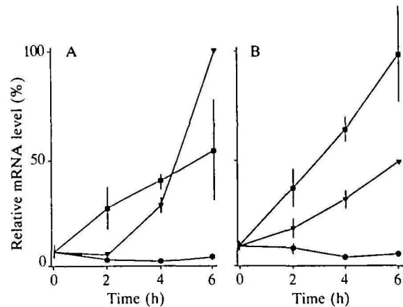
Fig. 2. The effects of different cyclic AMP stimulation regimes on CP-2 mRNA levels. Vegetative cells (A) and aggregation-competent cells (B) were incubated in PB without cyclic AMP (●), with 30 nM pulses of cyclic AMP every 6 min (▼) or with 30 \mu\text{M} -cyclic AMP added every hour (■). After 2, 4 and 6 h RNA was isolated, size fractionated and probed with PDD8 cDNA. Values of densitometric scans of specific RNA bands are expressed as percentage of the value of pulse-induced cells at 6 h incubation. The means and S.E.M. of data from three to six experiments are presented.
