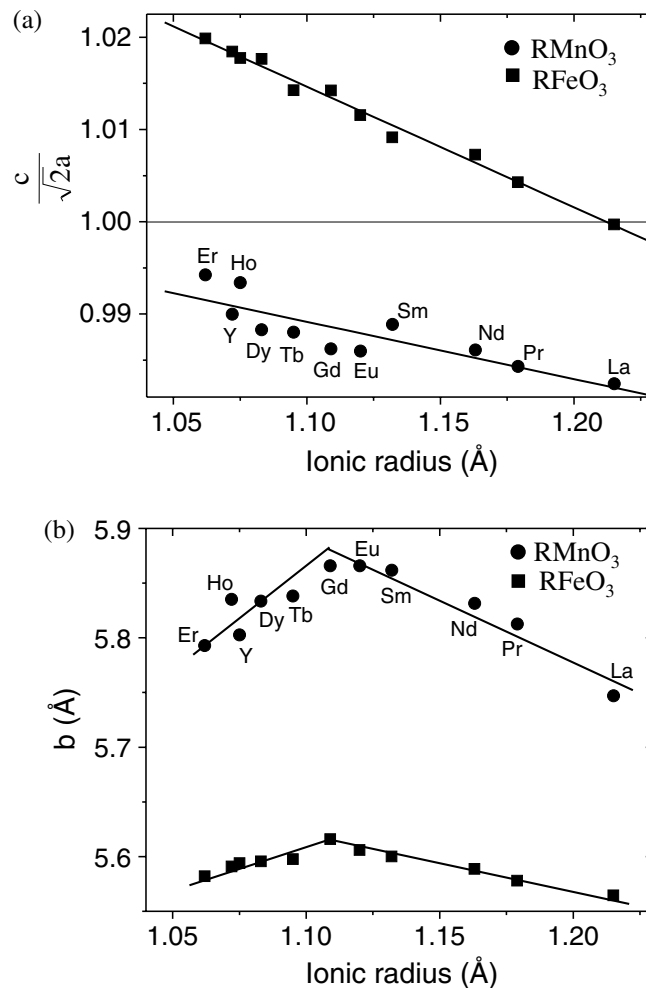
Figure 6. (a) Lattice parameter c/(\sqrt{2}a) ratio and (b) b for \text{RMnO}_3 [6, 7] and \text{RFeO}_3 [14, 17] versus the R-ionic radius. The O' structure shows c/(\sqrt{2}a) < 1 and O structure shows c/(\sqrt{2}a) > 1 .
