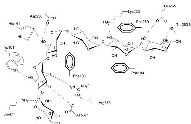
Fig. 2. Schematic overview of the interactions between T. thermosulfurigenes CGTase and a maltohexaose inhibitor bound from subsites -3 to +3 [34]. The interactions at subsite +3 are weak (3.6 Å). For clarity, not all interactions at subsites -1 and +1 are shown.
