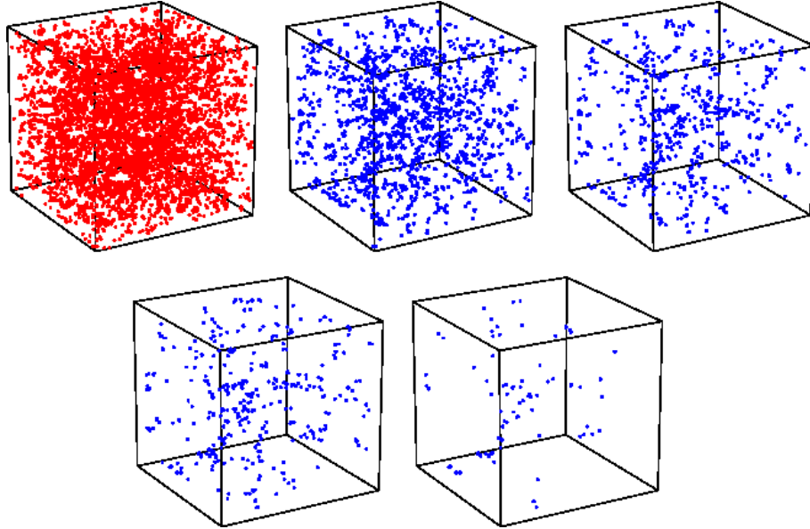
Figure 49. Selections of vertices from a full sample of vertices. Depicted are the (100%) full sample (top left), and subsamples of the 25%, 10%, 5% and 1% most massive vertices (top centre, top right, bottom left, bottom right). Note how the richer vertices appear to highlight ever more pronounced a filamentary superstructure running from the left box wall to the box centre. From: Van de Weygaert 2002a.
