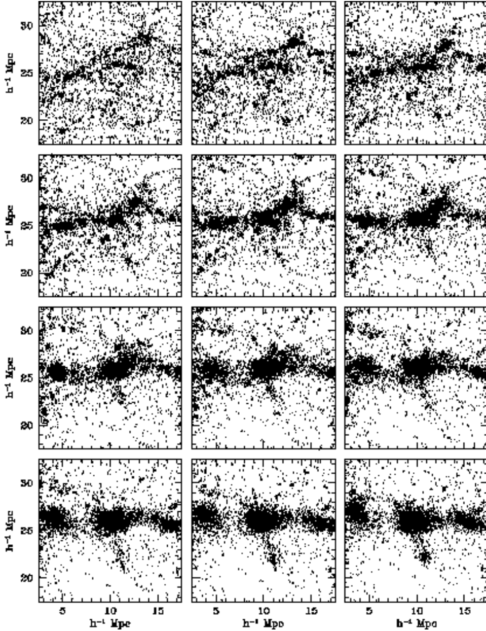
Figure 28. Gravitational Instability: hierarchical assembly of a filamentary structure. Focussing in on a small 15 \times 15 \times 15 h^{-1} \text{Mpc} region of a P^3M N-body simulation of structure formation in a SCDM scenario ( \Omega_0 = 1.0 , H_0 = 50 \text{ km/s/Mpc} ), from the 100 h^{-1} \text{Mpc} box 128^3 simulation shown in Fig. 12. Time is running from top left to bottom right, from a = 0.1 to a = 1.0 . Notice how small-scale clumps aggregate into ever larger haloes, all arranged along a roughly filamentary configuration (oriented horizontally).
