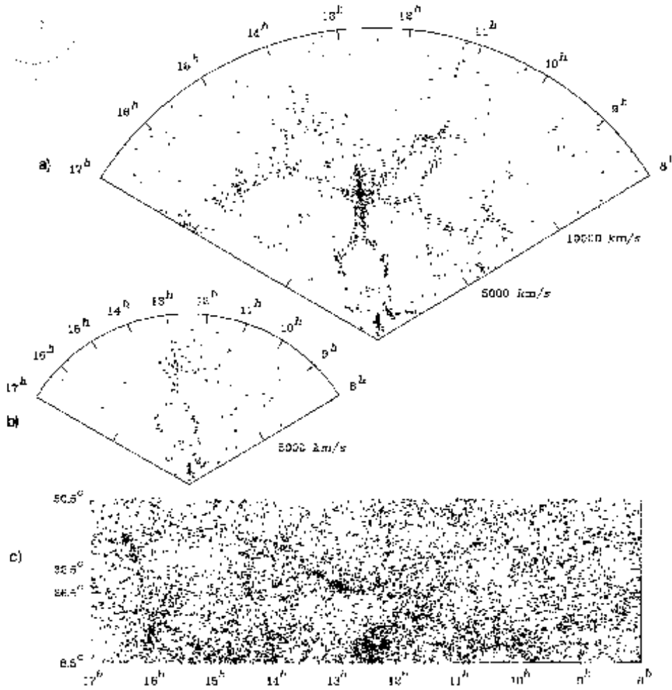
Figure 3. The revelation of the cosmic foam. The first published “Slice of the Universe” from the CfA2 survey, by de Lapparent, Geller & Huchra (1986). It comprises all galaxies with an apparent magnitude m \leq 15.5 in a narrow 6^\circ slice in a region towards the Coma Cluster ( (\alpha, \delta) \approx (13^h, 27^\circ) , sec ). This stereological sampling of the galaxy distribution represents a highly efficient method to obtain an impression of the overall spatial pattern. The result was the at first surprising finding of the apparently idiosyncratic cellular galaxy distribution. Note that the shallower CfA1 survey (cf. b), probing to m < 14.5 at hindsight contained a hint for these nontrivial patterns, be it not yet sufficiently convincing. Rightfully, this slice may be seen as a historic document, being a turning point for our view of the Universe’s structure. Courtesy: V. de Lapparent, M. Geller & J. Huchra. Reproduced by permission of the AAS.
