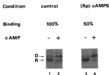
FIG. 3. Effect of (R p )-cAMPS on down-regulation and receptor modification. cAMP receptors were down-regulated by incubating cells for 15 min with 100 μM (R p )-cAMPS. Control cells were not exposed to (R p )-cAMPS. Cells were washed with ice-cold Mes, and incubated for 15 min with 0.5 μM cAMP + DTT. Lanes 1 and 2, control cells; lanes 3 and 4, cells with down-regulated receptors; lanes 1 and 3, cells immediately after washing in Mes buffer; lanes 2 and 4, cells after a subsequent incubation with 0.5 μM cAMP + DTT. cAMP binding was measured immediately after washing of cells with Mes buffer. Cells with down-regulated receptors by (R p )-cAMPS show 50% ± 8 of [ 3 H]cAMP binding.
