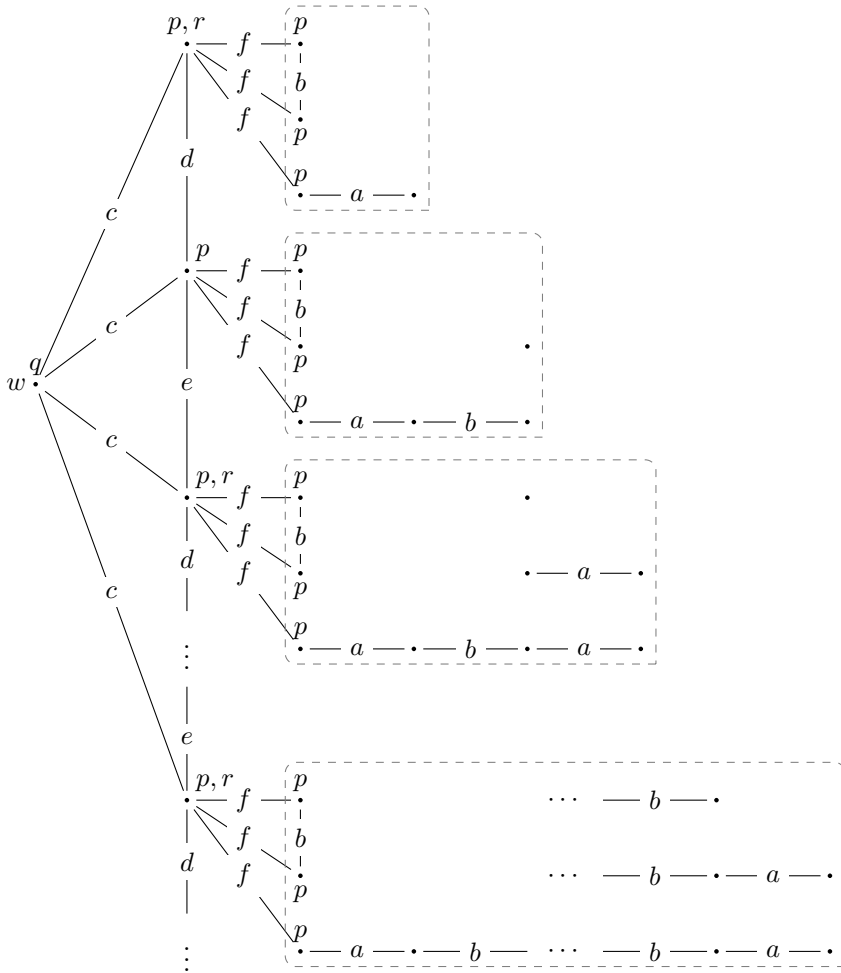
Figure 4.2: The model \mathcal{M}_\psi . Some accessibility arrows are not drawn.
