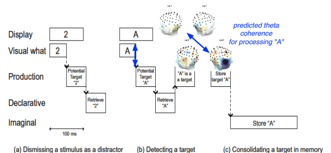
Figure 1: Example of predictions for neural correlates of interaction between modules in the attentional blink task (adapted from Taatgen et al., 2009). When the visual and later the production modules are identifying the letter “A,” there should be a specific increase in coherence in the theta band between the channels corresponding to the stimulus identification and target consolidation variates. These sets of channels were based on Figure 3.
