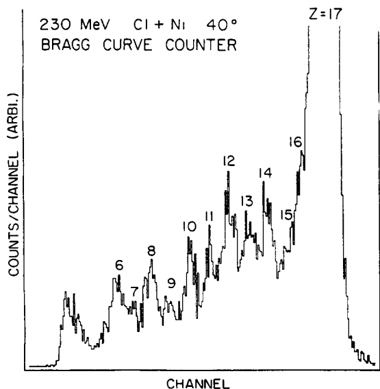
Fig. 7. Charge spectrum for the reaction ^{35}\text{Cl} + ^{58}\text{Ni} at 230 MeV.
