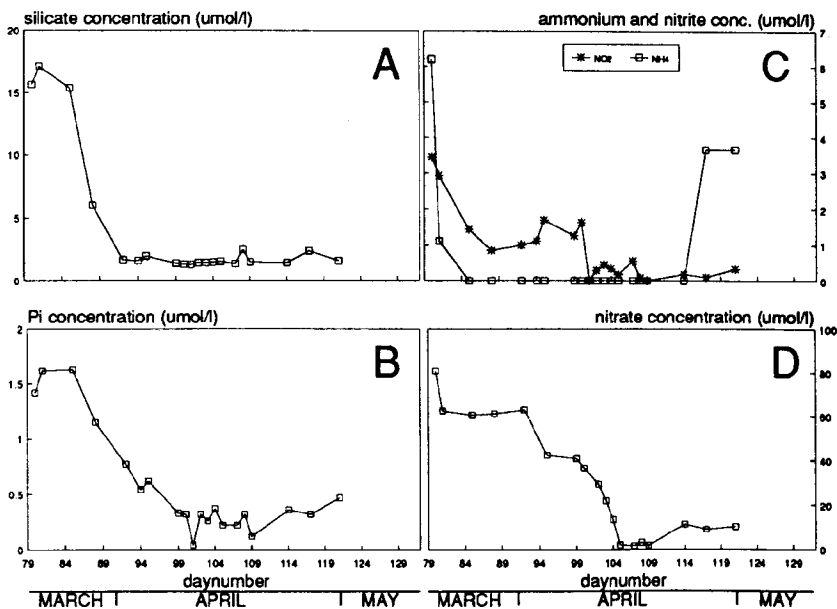
Fig. 1. Time course of the concentration of (A) silicate, (B) inorganic phosphate (Pi), (C) ammonium and nitrite, and (D) nitrate in the Marsdiep water during spring 1990
