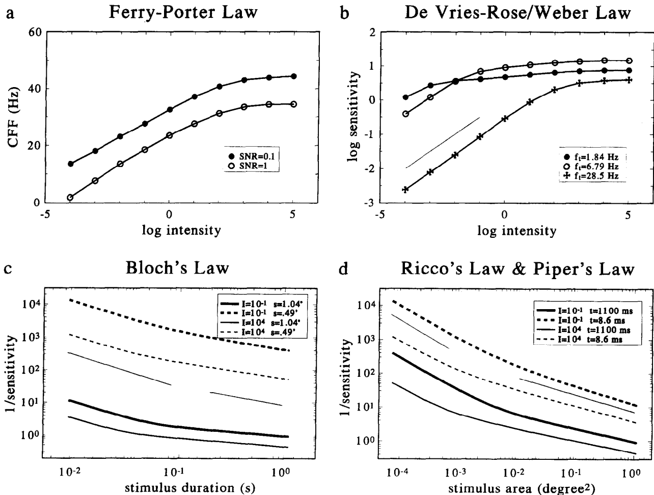
FIGURE 8. Several psychophysical laws as predicted by the theory. (a) Ferry-Porter law; CFF, critical flicker frequency; the figure shows the CFF for \text{SNR} = 1 and \text{SNR} = 0.1 . (b) de Vries-Rose/Weber law. The spatial frequency is 0 \text{ c/deg} . (c) Bloch's law for two intensities I and two stimulus sizes (the stimulus is a square of width s ). (d) Ricco's law and Piper's law for two intensities I and two stimulus presentation times t .
