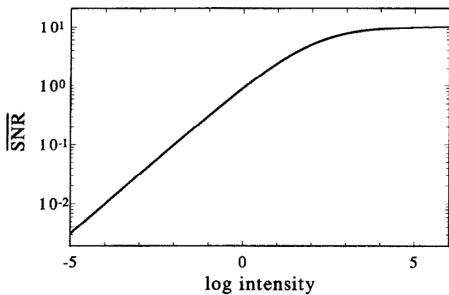
FIGURE 5. Resulting \overline{\text{SNR}} as a function of intensity according to equation (4).
