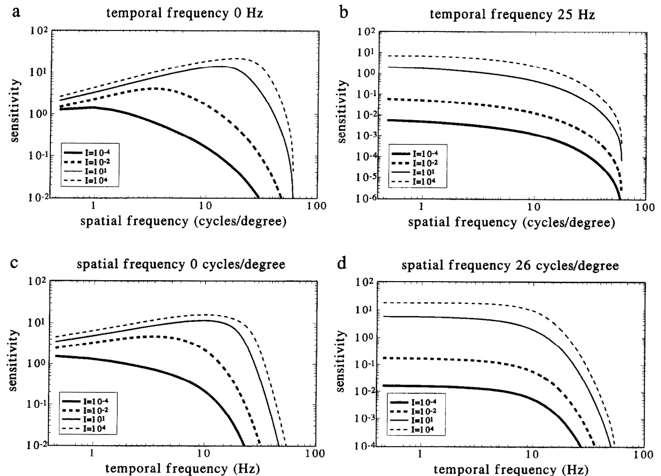
FIGURE 6. Contrast sensitivities at various spatial and temporal frequencies, and various intensities I . The intensity I is in arbitrary units, where I = 10 approximately corresponds to a retinal illuminance of 5 td.
