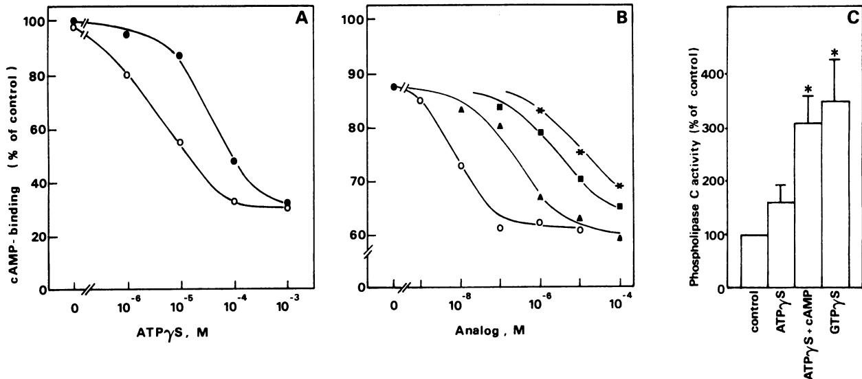
Fig. 3. Activation of G-proteins by NDP kinase. The activation of G-proteins was measured indirectly by analysing the effects of Mg^{2+} -ATP- \gamma S on agonist binding to surface receptors. (A) With (○) or without 10^{-5} M Sp-cAMPS (●). (B) 10^{-6} M ATP- \gamma S and cAMP (○), 2'-deoxy-cAMP (▲), Sp-cAMPS (■) and 8-Br-cAMP (*). (C) Activity of phospholipase C in the presence of 10^{-6} M ATP- \gamma S, 10^{-6} M ATP- \gamma S + 10^{-6} M cAMP or 10^{-5} M GTP- \gamma S. Data are expressed as a percentage of control (100% corresponds to 80 pmol/min/ 10^7 cells) and are the mean \pm SEM of four experiments in duplicate. *, significantly different from control with P < 0.05 .
