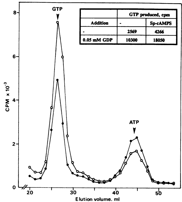
Fig. 2. Receptor-stimulated NDP kinase activity. HPLC profile of the produced [ ^{32} P]GTP from GDP and [ ^{32} P]ATP following the incubation of membranes with [ ^{32} P]ATP in the presence ( \bullet ) or absence ( \circ ) of the receptor agonist cAMP. Inset, c.p.m. GTP obtained under various conditions.
