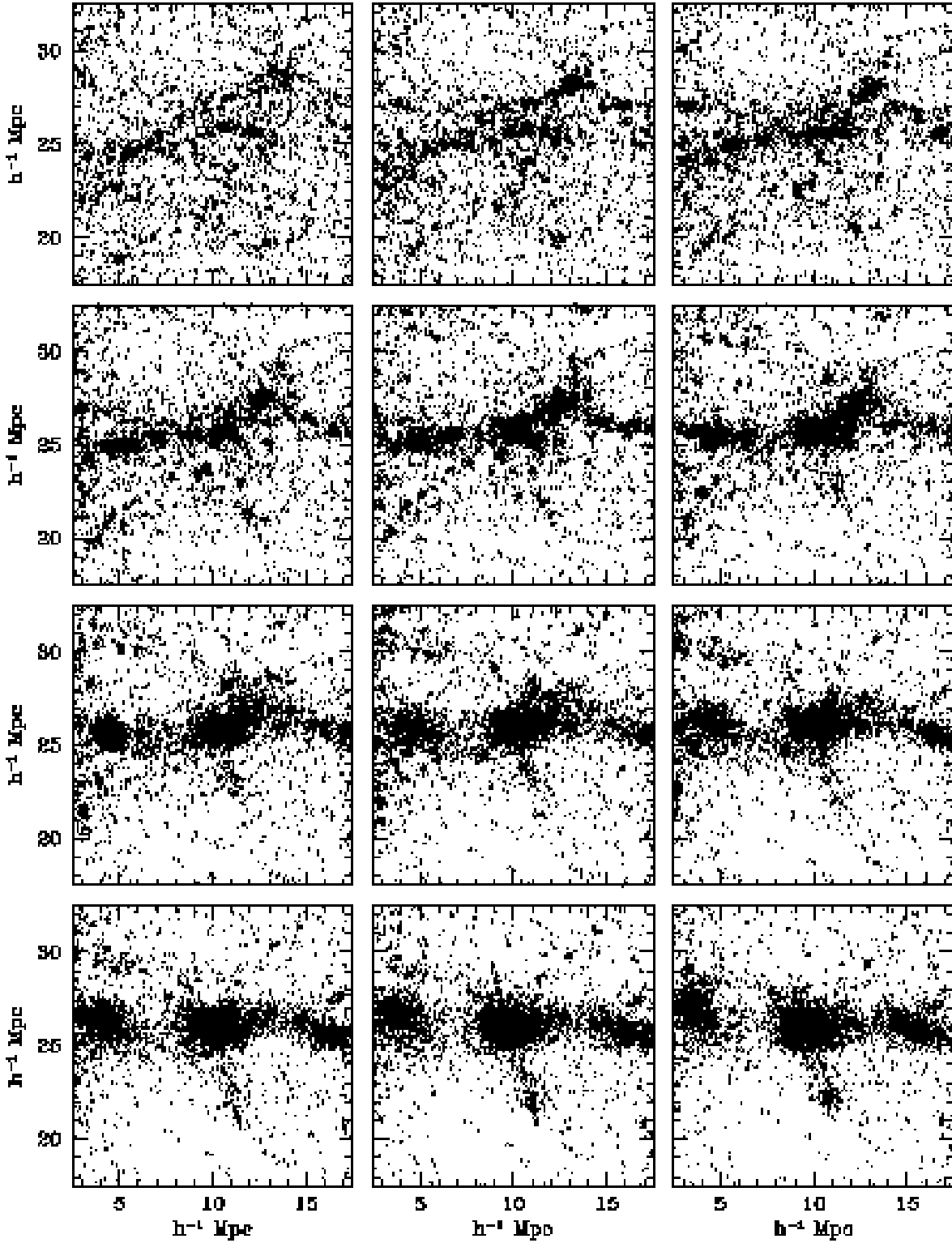
Figure 5. An illustration of gravitational clustering and collapse. The development of a small region in a 100h^{-1} \text{ Mpc} box, within the standard CDM scenario, is followed in a sequence of 12 time steps, going from left to right, top to bottom. The final timestep, bottom right, should correspond to the present epoch, a = 1 (From Van de Weygaert & van Albada 1996).
