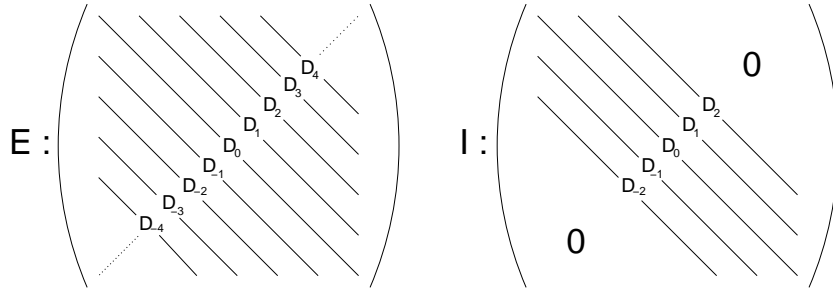
Figure 10: The interaction law \mathbf{I} (right) may be obtained from the external flow matrix \mathbf{E} (left) by omitting some off-diagonals (here only two diagonals on each side have been retained).
