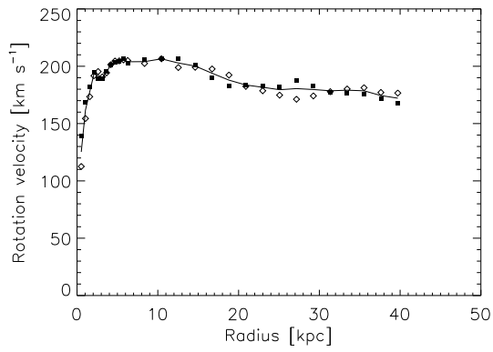
Fig. 10. Comparison between the rotation curve for the approaching side (filled squares) and receding side (open diamonds). The full line shows the rotation velocities obtained for the whole galaxy. We obtained these rotation curves using three values for the kinematical centre and two values for the systemic velocity (see Sect. 5). The two rotation curves are remarkably symmetric (compare with Fig. 7).
