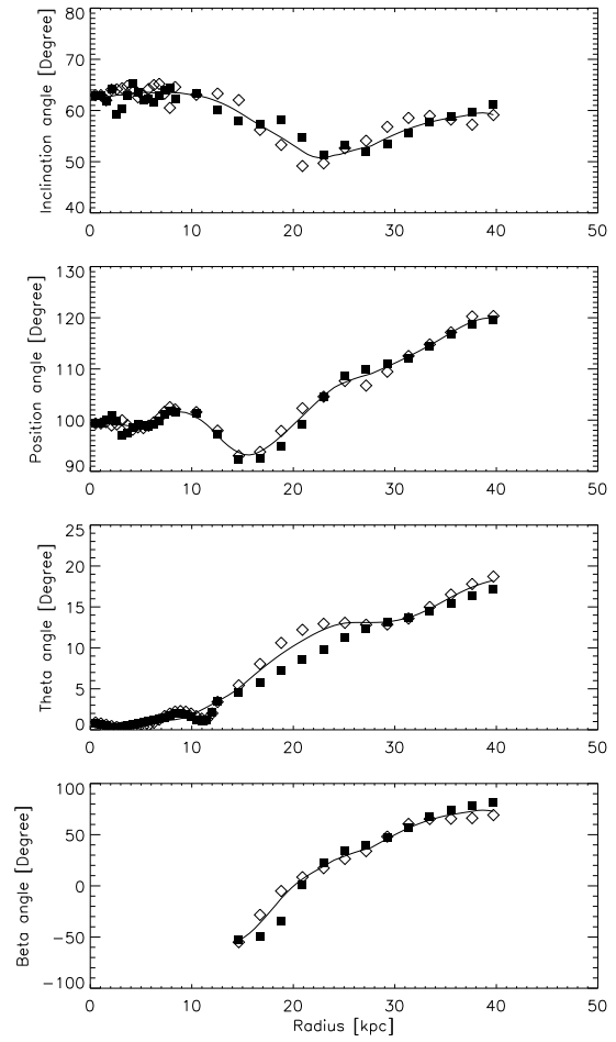
Fig. 9. Radial profiles of the warp parameters for NGC 5055, obtained using three values for the kinematical centre and two values for the systemic velocity (see Sect. 5). Filled squares show the approaching side, open diamonds the receding side, and the full line shows the parameters for the whole galaxy. Note the remarkable symmetry of the galaxy if compared with the same plots in Fig. 6.
