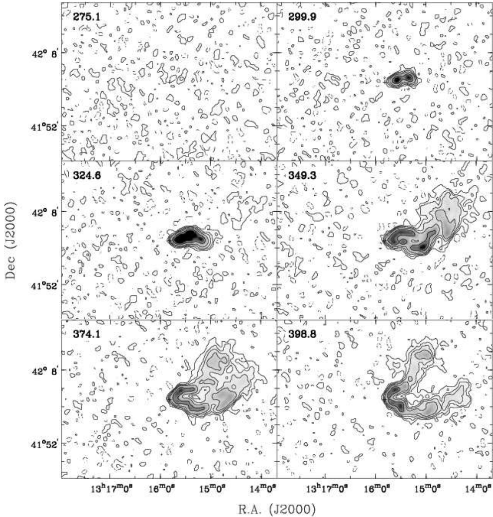
Fig. 3. HI channel maps of NGC 5055 at 67'' resolution (Hanning smoothed). Contours are -1.2 (dashed), 1.2, 3, 6, 12, 30, 60, 120, 300 mJy/beam; the r.m.s. noise is 0.6 mJy/beam. The heliocentric velocities (in \text{km s}^{-1} ) are shown in the upper left corner; the cross indicates the kinematical centre of the galaxy.
