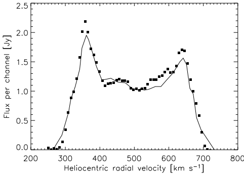
Fig. 2. Comparison between the global HI profile of NGC 5055 from this work (squares) and from single dish observations (full line) by Rots (1980).
