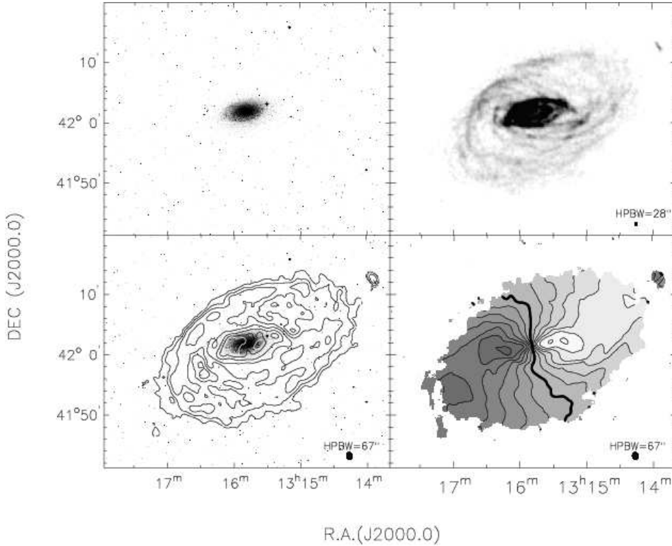
Fig. 1. Top left: Optical image (DSS) of NGC 5055. Top right: Total HI map at 28'' resolution. Bottom left: Total HI map at 67'' resolution overlaid with the DSS optical image; contours are 3.0, 6.0, 12.0, 20.6, 41.2, 82.4, 123.4 \times 10^{19} \text{cm}^{-2} . Bottom right: Velocity field at 67'' resolution; contours are separated by 30 \text{km s}^{-1} , and the thick line shows the systemic velocity (497.6 \text{km s}^{-1} ); the receding side is S-E.
