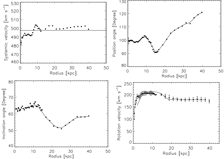
Fig. 5. Parameters for NGC 5055 obtained from the tilted ring model fit. In the top left panel the horizontal line shows the mean systemic velocity adopted in this work, v_{\text{sys}}=497.6 \text{ km s}^{-1} . The full lines in the plots for the position and inclination angles were obtained smoothing the data, in order to remove small-scale fluctuations. Bottom right panel: rotation curve from this work (filled squares) compared with the rotation curve (line) derived by Bosma (1978).
