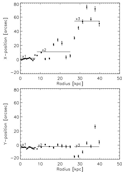
Fig. 8. Radial trend of the x (top) and y (bottom) position of the dynamical centre for NGC 5055. The horizontal lines indicate the three different values for the coordinates used in the tilted ring model fit described in Sect. 5.
