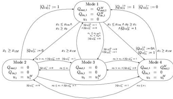
Fig. 3. Hybrid controller for Zone 1. Following standard convention, when the edge has two labels the first one represents the guard, the second one (denoted by :=) the reset. When no reset is present, then all the variables remain unchanged upon the transition. All the guards at the edges linking the three states at the bottom should include the clause \neg x_1 \geq x_{1M} , which is omitted for the sake of simplicity. For each mode (discrete state) only three representative values are indicated. The remaining values can be derived from Table 2 specialized to the case i = 1 .
