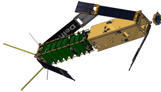
Fig. 5 Exploded view of the Delfi-C 3 three-unit CubeSat of the Delft University of Technology.
