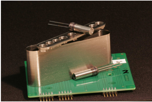
Fig. 4 Plenum, plate, gas generators and electrical interface before assembly – © H.J. Siemer (TNO).
