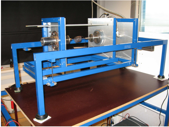
Fig. 3 Delft Aerospace Rocket Test Stand (DARTS).
