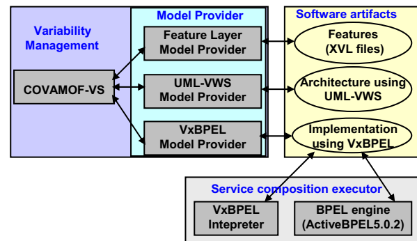
Fig. 5. The variability management platform for service compositions
