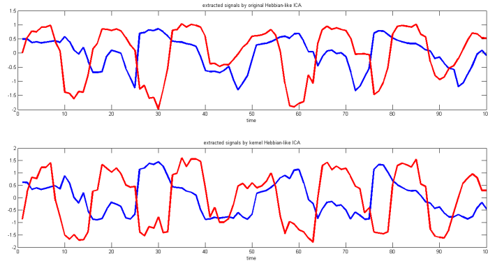
Figure 2: Estimated source signals by original Hebbian-like ICA based on the Euclidean inner product (top) and by the kernelized variant (bottom).
