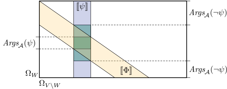
Fig. 2. The sets of arguments and counter-arguments of a hypothesis \psi obtained from the given premises \Phi . The sample space \Omega_W is a sub-space of the entire space \Omega_V = \Omega_W \times \Omega_{V \setminus W} .
