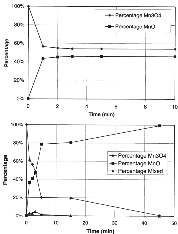
Fig. 2. Fraction of \text{Mn}_3\text{O}_4 and MnO precipitates as a function of annealing time in reducing atmosphere at 400°C (a) and 600°C (b).
