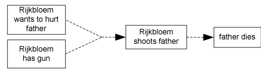
Figure 2: a small causal network
