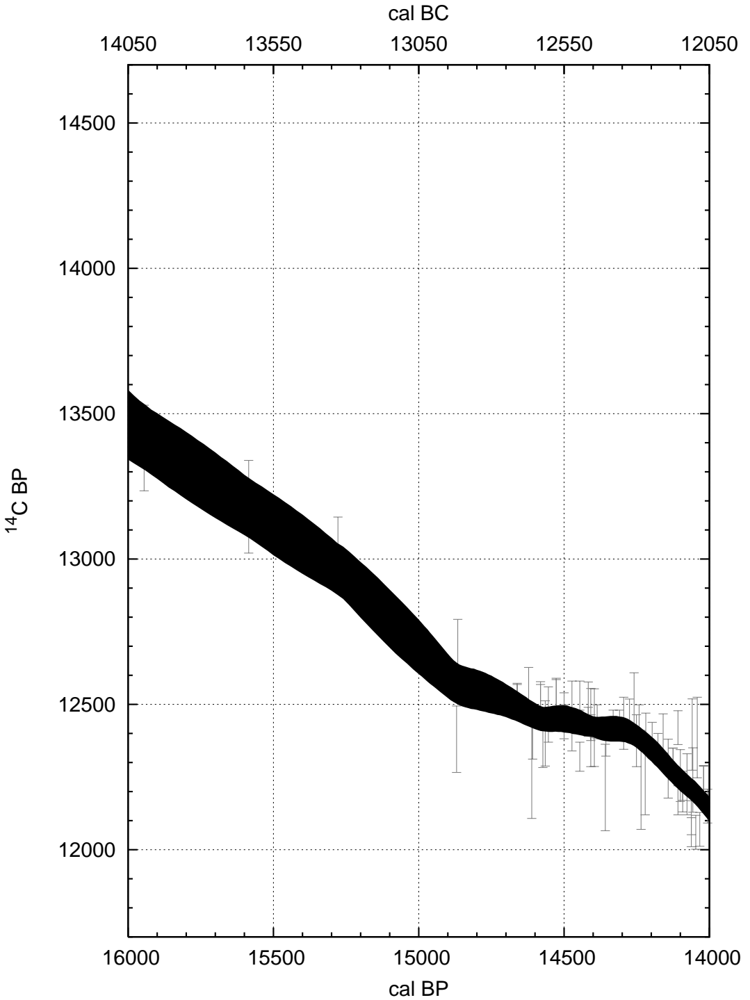
Figure A6 The IntCal04 terrestrial calibration curve (1-standard deviation envelope) and data with 1-standard deviation error bars in 14 C increased by the laboratory error multipliers described in the text. The uncertainty in the calendar ages is not shown, but is taken into account in the random walk model.
