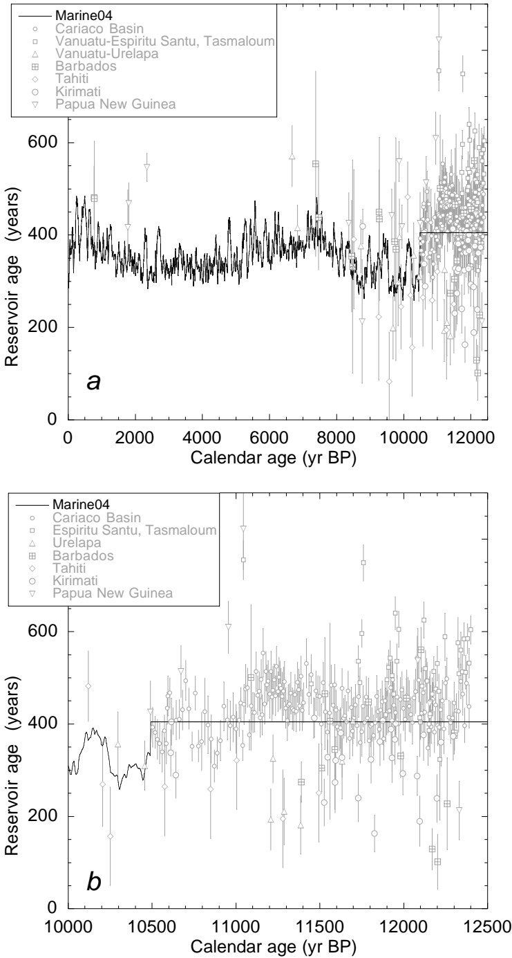
Figure 2 Site-specific reservoir corrections for the locations used in IntCal04 and Marine04. Sites include Cariaco Basin (Hughen et al., this issue); Vanuatu (Burr et al. 1998; Cutler et al., this issue); Barbados (Bard et al. 1998; Fairbanks et al., forthcoming); Tahiti (Bard et al. 1998); Kirimati (Fairbanks et al., forthcoming); and Papua New Guinea (Edwards et al. 1993; Cutler et al., this issue). (a) Reservoir corrections from 0–12.5 cal kyr BP. Marine04 reservoir R changes from 0–10.5 due to shifts in atmospheric ^{14}\text{C} production, but is held constant beyond 10.5. (b) Blow-up of interval of greatest marine-terrestrial data overlap. Slight but coherent changes in reservoir age through time are likely due to real changes in oceanographic conditions (see text).
