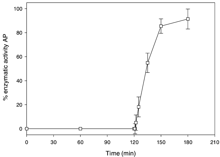
Fig. 2. Amount of enzymatic activity that was found in the dissolution test of inulin/BIAP (19/1, w/w), coated tablets. The pH was increased to 6.8 after 2 h; 100% activity is defined as the level of activity that is expected based on the amount of BIAP present in the tablet.
