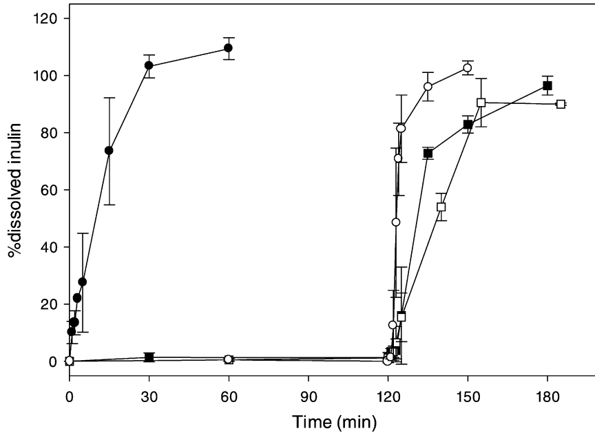
Fig. 1. In-vitro dissolution testing of tablets measured as dissolved inulin; (●) inulin/BIAP (19/1, w/w), non-coated; (■) inulin, coated; (□) inulin/BIAP (19/1, w/w), coated; (○) inulin/primojel (95/5, w/w), coated. The pH was increased to 6.8 after 2 h.
