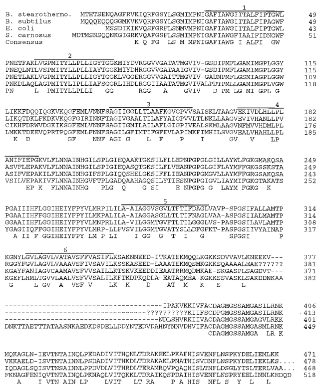
FIG. 4. Multiple amino acid sequence alignment of the B. stearothermophilus IICB Mtl , the IICB part of the IICBA Mtl s of B. subtilis (1) and E. coli (13), and the S. carnosus IICB Mtl (7). Identical amino acids are given in the consensus sequence. Membrane-spanning regions of the E. coli enzyme predicted by PhoA fusions (30) are indicated by numbered lines above the sequence. Probable sequence errors in the B. subtilis sequence (accession number D38161) were corrected by a deletion of a guanine at position 1068 and an adenine at position 1490 and an insertion of an alanine at position 1119. Also, in the linker region between the C and B domains, a frame shift probably caused by a deletion occurs. Because of the low similarity in this part of the sequence, the position of this deletion is not clear. This part is indicated with question marks.
