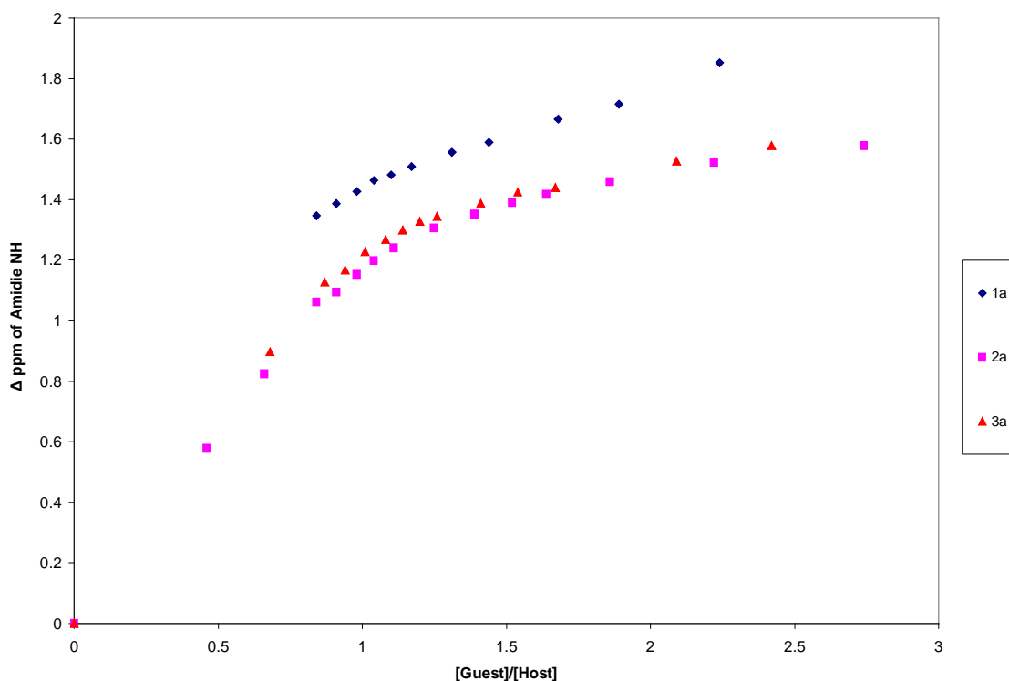
Figure 5: Comparison of binding of bisamidopyrrolyl carbazole receptors with phosphate
