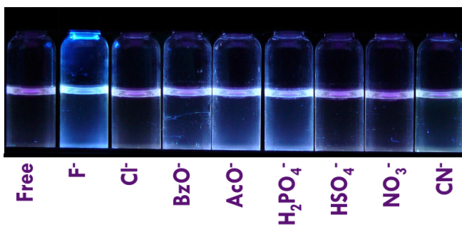
Figure 4: Fluorescence of 3a with various anions
