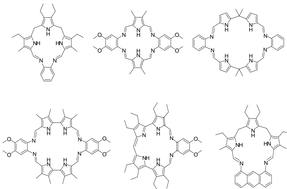
Figure 2: Examples of some expanded porphyrins
