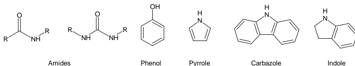
Figure 1: Some natural hydrogen bond donors
