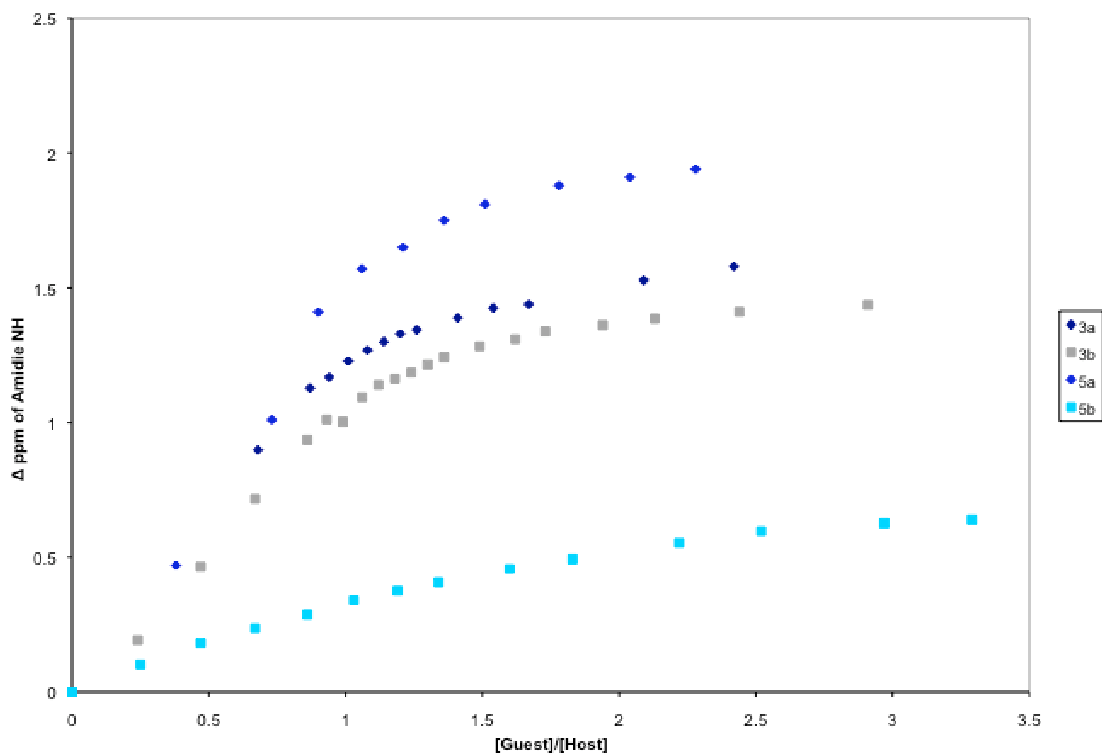
Figure 3: Comparison of binding between receptors 3 and 5 with phosphate
