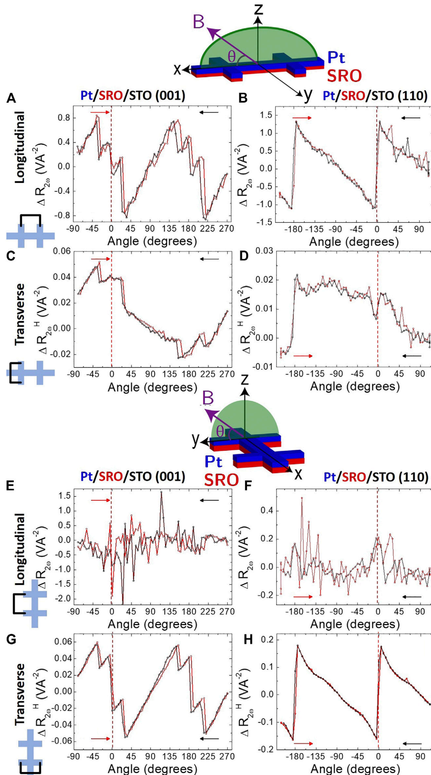
FIGURE 3 | Second harmonic angular measurements for \text{SRO}_{001} (left) and \text{SRO}_{110} (right). Data for xz sweeps are shown in (A,B) for the longitudinal resistance and in (C,D) for the transverse resistance. The yz scans are shown in (E,F) for the longitudinal resistance and in (G,H) for the transverse resistance. The angle ( \theta ) of the magnetic field ( B ) is indicated with respect to the in-plane direction. \Delta R indicates the change in resistance with respect to when the field is applied out-of-plane. Red and black lines are used to indicate the trace (increasing angles) and retrace (decreasing angles) scans respectively.
