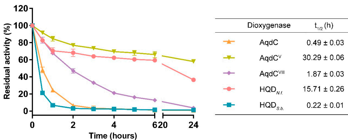
Figure 2. Effect of temperature on the enzymatic activity of PQS dioxygenases. Enzyme solutions (0.2 mg mL -1 ) in PBS (pH 7.5) were incubated at 37 °C, and residual catalytic activities of samples withdrawn at appropriate time intervals were measured using the standard enzyme assay. The catalytic half-life ( t_{1/2} in [h]; period required for the enzymatic activity to decrease to half of its initial value) was determined by fitting the data to the one-phase exponential decay model, with the plateau parameter adjusted to a constant value of zero, using GraphPadPrism 6 software. Data represent the average ± SD from triplicate experiments.
