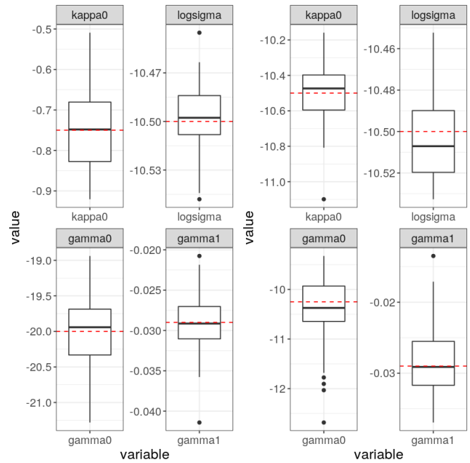
Fig. 7. Fixed \kappa_1 . Box plots for estimated parameters in 50 realizations of the constant (left) and quadratic (right) rate model. Red dashed lines indicate the true parameters.
