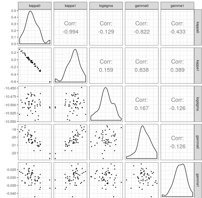
Fig. 10. Pairwise scatter plots for the parameter estimates of 50 realizations of the constant rate model.
