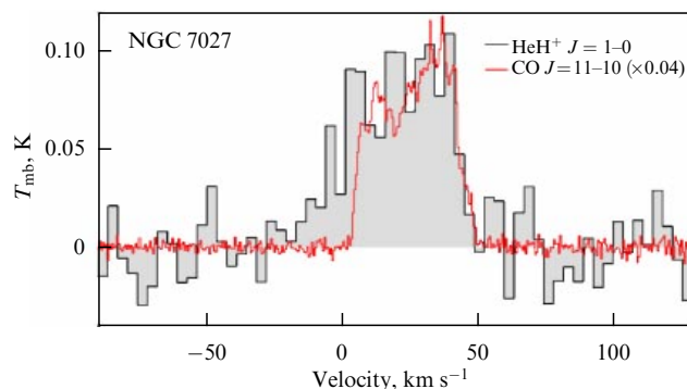
Figure 20. (Color online.) Spectrum of the rotational \text{HeH}^+ ( J = 1 - 0 ) transition measured with the upGREAT (upgraded German Receiver for Astronomy at Teraherz frequencies) instrument aboard SOFIA in the direction of NGC 7027. For comparison, shown is the CO ( J = 11 - 10 ) line arising in a dense molecular shell near the ionization front from which the \text{HeH}^+ emission is expected. (Figure from paper [270].)
