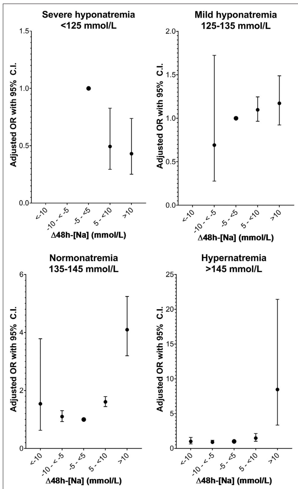
Figure 1. Association between in-hospital mortality and \Delta 48\text{ hr-[Na]} for ICU patients categorized by first serum sodium measurement at ICU admission. The adjusted odds ratios (ORs) for risk of in-hospital mortality using logistic regression. Adjusted for age, sex, and Acute Physiology and Chronic Health Evaluation-IV predicted mortality. \Delta 48\text{ hr-[Na]} of -5 to 5 mmol/L was used as reference category. \Delta 48\text{ hr-[Na]} = difference between mean of sodium measurements 24–48 hr after ICU admission and first serum sodium at admission in mmol/L.
