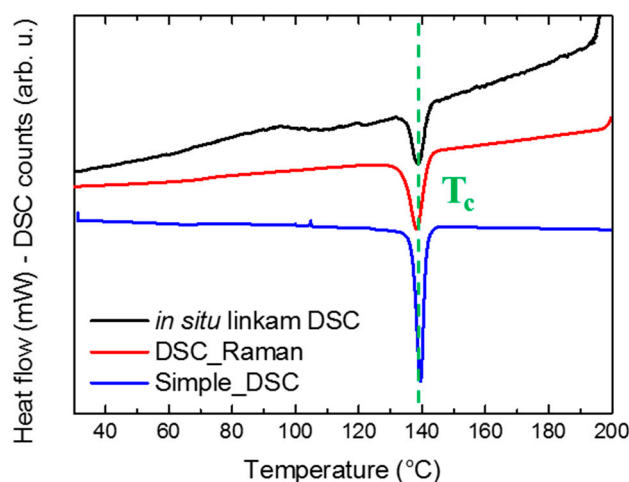
Figure 3. Comparison of the thermograms obtained by the Linkam DSC600 setup (X-rays and Raman laser on), the Q200 TA DSC-Raman setup (Figure S2A available in the supplementary material document) and a single Q200 TA DSC profile. Slight discrepancies in the crystallization temperature were observed, as well as a slight drift in the baseline.
