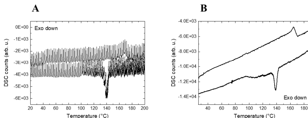
Figure 2. Linkam DSC profile of the cooling and second heating ramps of the PVDF sample during the simultaneous SAXS/WAXS coupled to the Linkam DSC combined with the Raman spectrometer with the activated laser shutter (A) and with the deactivated laser shutter (B).
