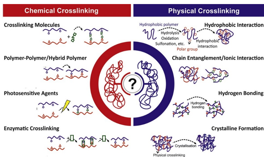
Figure 2. Schematic representation of various types of physical and chemical crosslinking in hydrogels (adapted from [22], CC-BY license).
