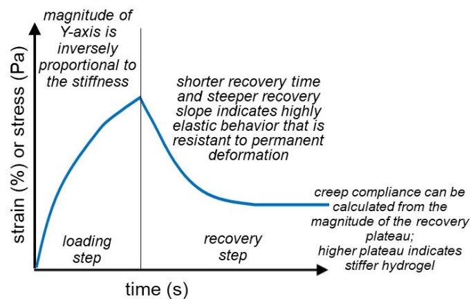
Figure 8. Creep recovery tests show the amount of applied strain a hydrogel can withstand and how the structure of the hydrogel recovers upon removal of this applied strain.
