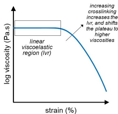
Figure 4. Strain sweep or amplitude sweep in hydrogels shows the linear viscoelastic region (LVR) as well as the threshold strain required above which shear thinning behavior is observed.
