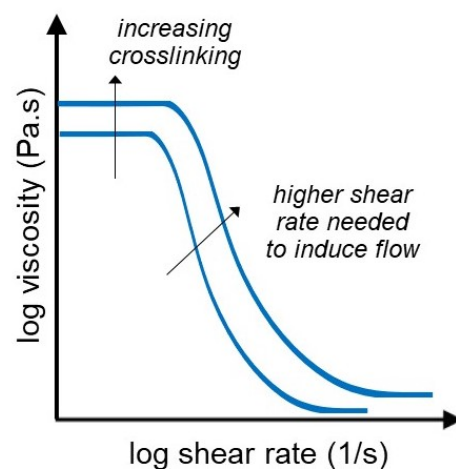
Figure 3. Schematic graph showing the flow behavior of hydrogels, represented by viscosity as a function of shear rate.
