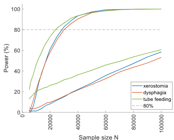
Fig. 3. Statistical power of showing an independent relation between toxicity and voxel-wise product of D and LET_d ( D-LET_d ) for an assumed RBE-LET_d slope c of 0.04 or 0.1 (keV/\mu m)^{-1} . Each toxicity has two line plots associated with it. The lower and higher estimates were for 0.04 and 0.1 (keV/\mu m)^{-1} respectively.
