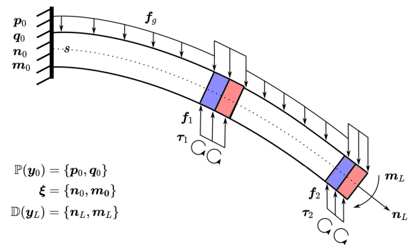
Fig. 2. Proximally fixed, and distally free-floating, discretely magnetized continuum manipulator (CM), characterized by a centerline parameter ( s \in [0, L] ), subject to distributed magnetic forces ( \mathbf{f}_m(s) ) and torques ( \boldsymbol{\tau}_m(s) ), and gravitational forces ( \mathbf{f}_g(s) ). Material cross-sections along s are characterized by a position ( \mathbf{p}(s) ), orientation quaternion ( \mathbf{q}(s) ), internal force ( \mathbf{n}(s) ), and internal moment ( \mathbf{m}(s) ); collected in state parameter vector ( \mathbf{y}(s) ). Known proximal and distal boundary conditions are denoted as \mathbb{P}(\mathbf{y}_0) and \mathbb{D}(\mathbf{y}_L) , respectively. Unknown proximal states are collected in an optimization vector ( \boldsymbol{\xi} ).
