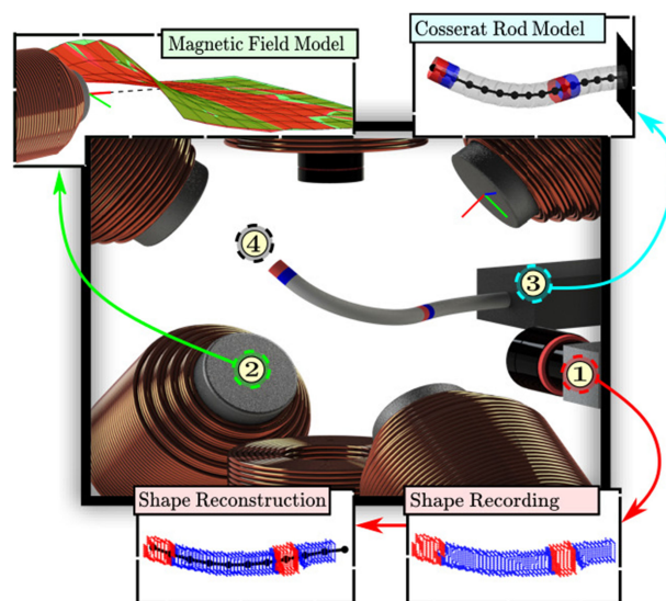
Fig. 1. In this study we use BigMag, an array of 6 mobile electromagnetic coils [12], to perform closed-loop orientation control of two permanent magnets carried by a continuum manipulator (CM). ① Shape reconstruction of the CM is performed with a stereo vision setup. ② A model of the magnetic field then predicts exerted magnetic wrenches on the CM. ③ With Cosserat rod theory a quasi-static forward model of the CM is produced. ④ This model is used to predict changes in magnet orientations, due to changes in the currents and positions of the electromagnets, in order to actuate the CM.
