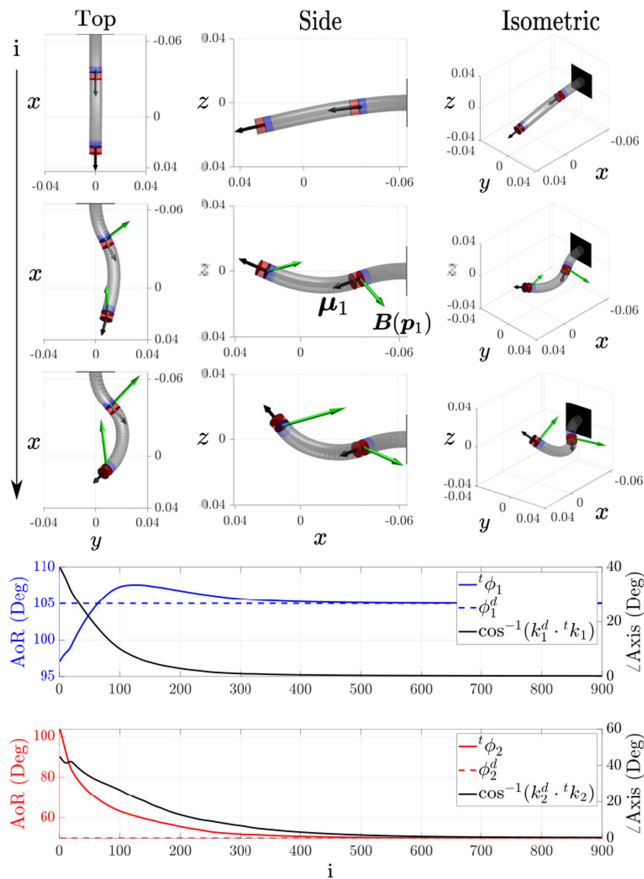
Fig. 6. Top, side, and isometric views of CM shapes at starting, intermediate, and final iteration numbers (i) with dimensions shown in meters. Trajectories of the theoretical magnet angles of rotation (AoR, {}^t\phi_m ), for the proximal and distal magnet, are given in blue and red, respectively. Also, the trajectories of the angular distances between the theoretical and desired axes of rotation ( \angle Axis ) are shown.
