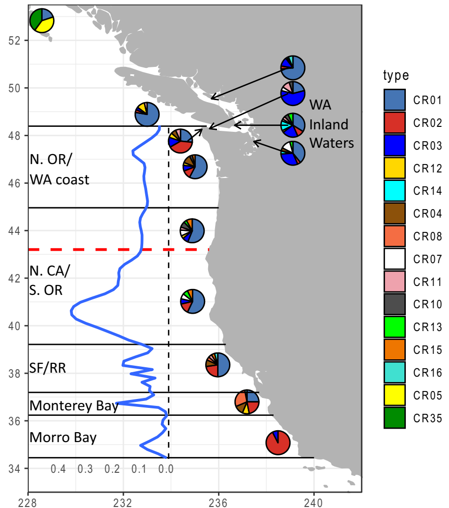
FIGURE 5 Pie charts representing frequencies of haplotypes represented by \geq 5 samples in the stratum, plus two haplotypes (CR05, CR35) that were found only in the BC strata, in two samples each (out of five in total). Relative porpoise density estimates (porpoise per kilometre surveyed) is plotted by latitude, averaged across multiple survey periods (blue line). The current US stocks are named and boundaries are represented by horizontal black lines (as in Figure 1). The proposed boundary location for splitting the Northern California/Southern Oregon stock into two stocks is shown with a dashed red line
