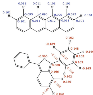
Fig. 4 Point charge values used for the QM/MM calculations for tetracene (top) and DPBF (bottom). Due to symmetry, only equivalent charges are shown.
