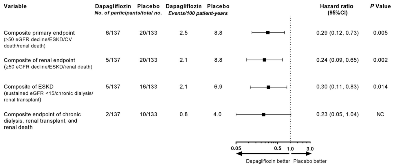
Figure 2 | Forest plot of the key endpoints. Estimated glomerular filtration rate (eGFR) is expressed as ml/min per 1.73 \text{ m}^2 . CI, confidence interval; CV, cardiovascular; ESKD, end-stage kidney disease; NC, not calculable.
