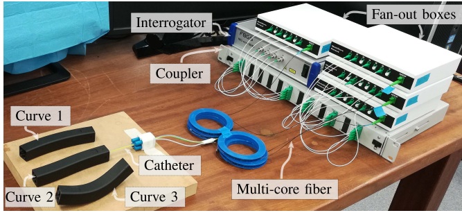
Fig. 5. Setup for Experiment 1. The catheter is sensorized with four multi-core fibers that have fiber Bragg gratings (FBG); each catheter segment has one fiber. The experiment utilizes four multi-core fibers, fan-out boxes, interrogator, coupler, catheter, and three molds.
