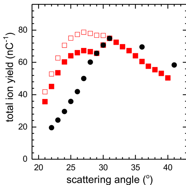
Fig. 4. Scattering-angle dependence of measured total ion yields (black symbols) for 7 keV \text{Kr}^+ ions on Cu at an incidence angle \psi of 15^\circ . The closed red squares indicate total scattering yields obtained from SRIM (scaled at 31^\circ ), which at angles below 30^\circ lack contributions from SC events. The open red squares show the SRIM data after correction for the missing SC events at angles below 30^\circ . The correction is based on assuming a constant SC fraction (see Fig. 5). (For interpretation of the references to color in this figure legend, the reader is referred to the web version of this article.)
