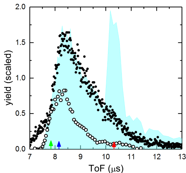
Fig. 6. Comparison of the experimental ToF spectrum (closed black symbols) of backscattered particles (ions and neutrals) and the SRIM predictions (cyan) for 5 keV \text{Kr}^+ ions on a Cu target at a scattering geometry of (\psi, \theta) = (15^\circ, 40^\circ) . The open black symbols represent the measured ion energy spectrum converted to time scale. The ToF positions of single and symmetric double scattering are marked by red and blue arrows, respectively. The green arrow indicates the position of primary Cu recoils in the ToF spectrum. (For interpretation of the references to color in this figure legend, the reader is referred to the web version of this article.)
